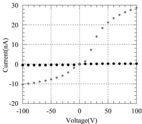
FIGURE 3 Photocurrent response at 31°C in the smectic E phase. of 8-PNP-4. ( d = 15 \mu\text{m} , S = 16 \text{ mm}^2 , ITO/ITO)
