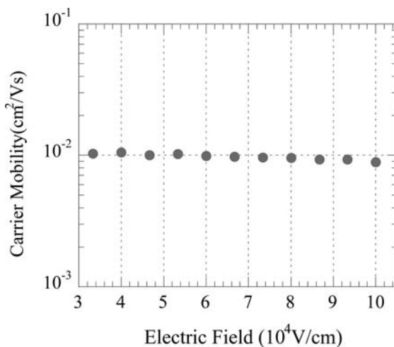
FIGURE 6 Electric field dependence on hole carrier mobility at 31^\circ\text{C} in the smectic E phase of 8-PNP-4. ( d = 15 \mu\text{m} , S = 100 \text{ mm}^2 , ITO/ITO)
