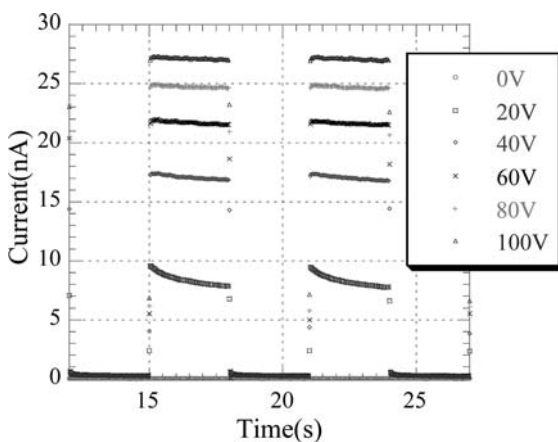
FIGURE 2 Photocurrent response at 31°C in the smectic E phase of 8-PNP-4. ( d = 15 \mu\text{m} , S = 16 \text{ mm}^2 , ITO/ITO)
