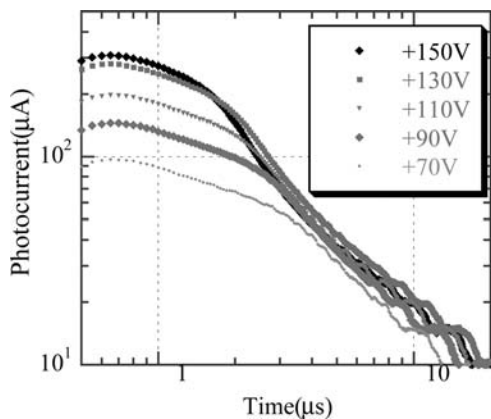
FIGURE 4 Transient photocurrent curves at 31°C in the smectic E phase of 8-PNP-4. ( d = 15 \mu\text{m} , S = 100 \text{ mm}^2 , ITO/ITO)
