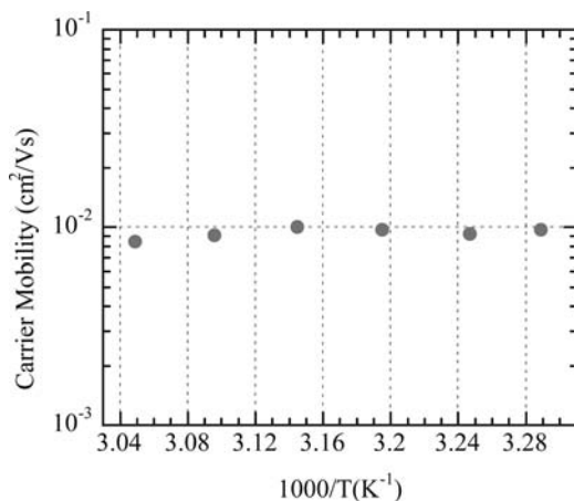
FIGURE 5 Temperature dependence on hole carrier mobility in the smectic E phase of 8-PNP-4. ( d = 15 \mu\text{m} , S = 100 \text{ mm}^2 , ITO/ITO)
